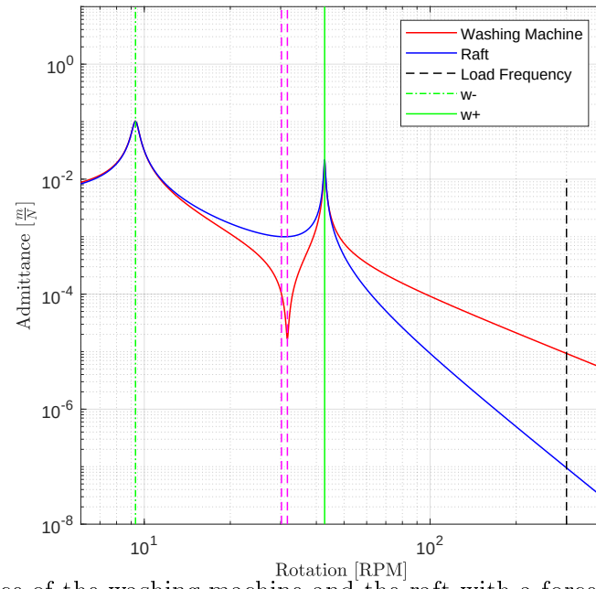
Figure 7: Admittance of the washing machine and the raft with a force on the washing machine.
